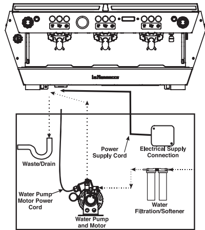
Fig. 2 - Installation Guide
